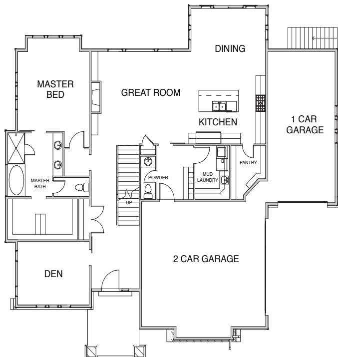
MAIN FLOOR
