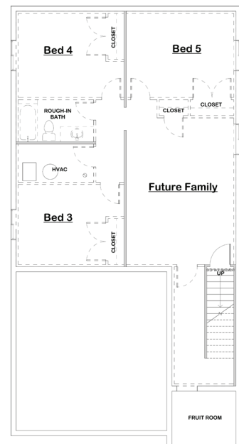
BASEMENT
